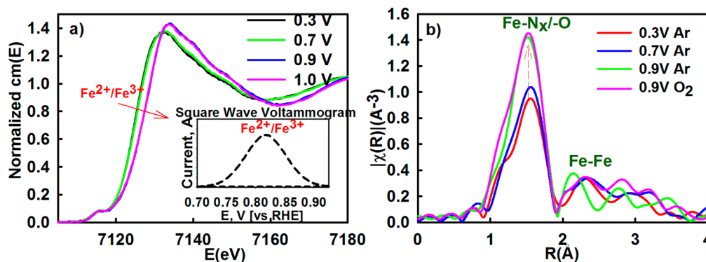
Figure 3. (a) Potential dependent normalized Fe K-edge XANES spectra with corresponding redox peak transition shown in inset as a background-subtracted square wave voltammogram profile collected in oxygen-free 0.1 M HClO 4 . (b) Fourier Transform of the extended region of the XAS spectra collected in situ at Fe K-edge (7112 eV) of PVAG-Fe catalyst.
